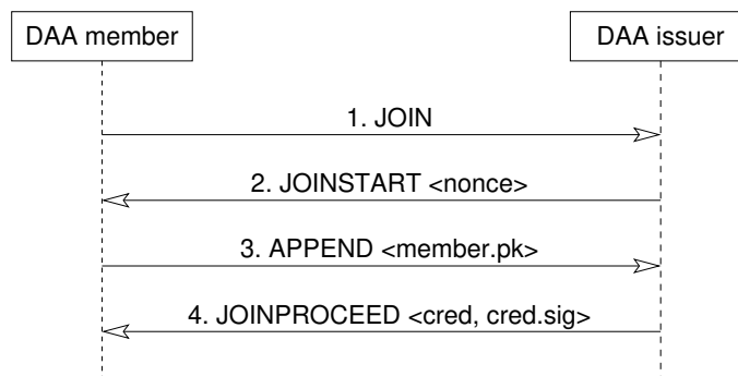
Figure 4.3: Protocol to add a new member to the issuer's DAA group
