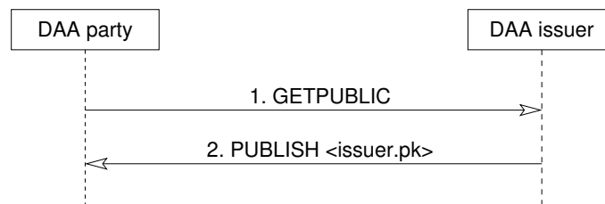
Figure 5.2: Protocol to get the issuer's public key
