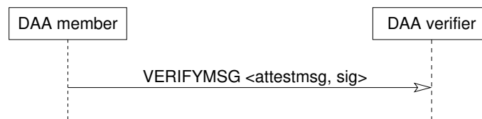
Figure 5.4: Protocol to send an attestation message to the verifier
