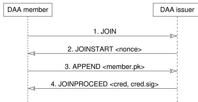
Figure 5.3: Protocol to add a new member to the issuer's group
