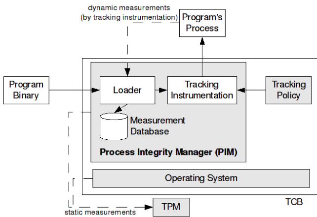
Figure 1: Architecture of DynIMA
