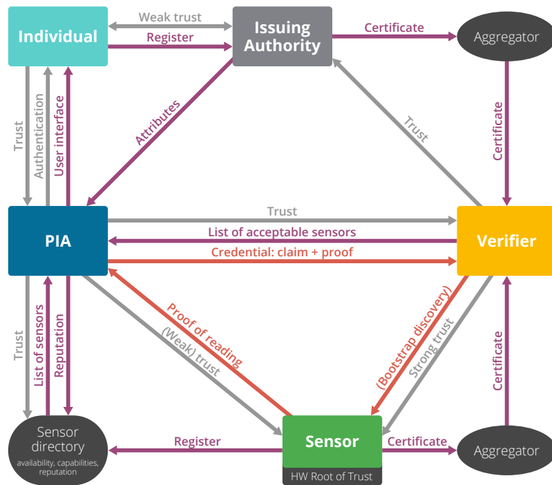
Figure 1.1: Overview of the Digidow network with its interactions [18]
